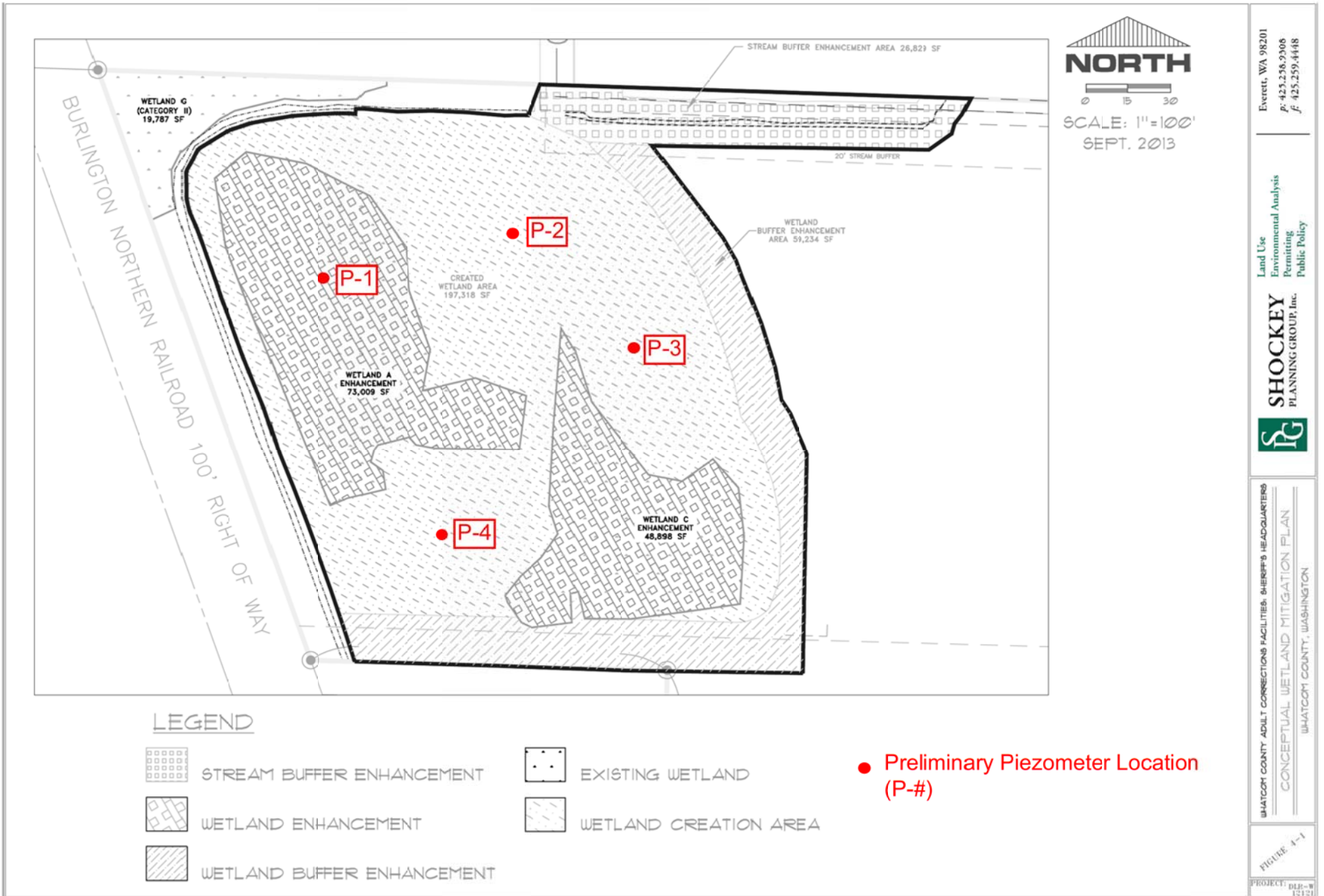
Figure 2. Preliminary Proposed Piezometer Locations
